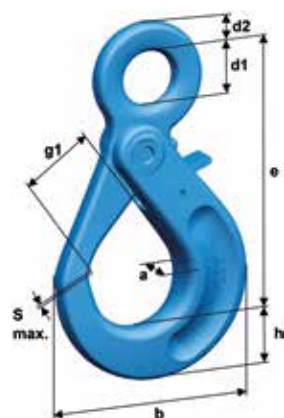
LHWP Safety hook
