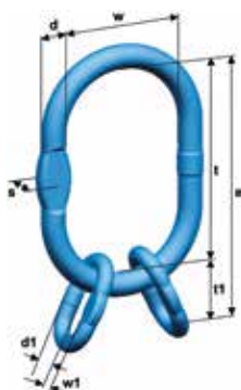
VMWP Enlarged master link assembly
