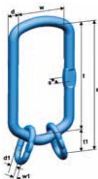
VLWP 2/4 Oversize master link assembly
